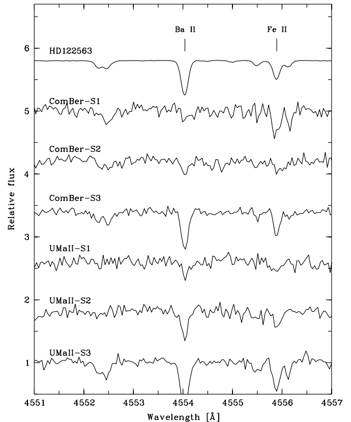
Figure 2. Spectral region around the Ba line at 4554 Å for the program stars. The Ba and other metallic lines are detected but have significantly different line strengths in each spectrum, confirming the large spread in abundances of these elements in both UMa II and ComBer.
