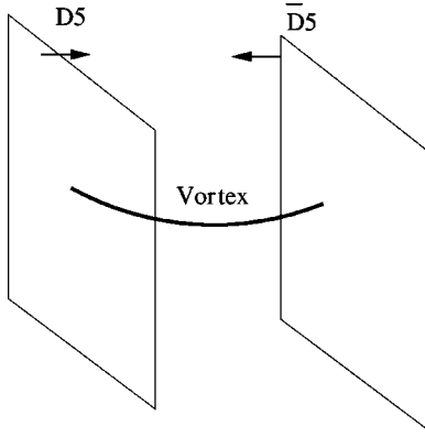
FIG. 1. This is a depiction of the annihilation of two parallel coincident D5- \bar{D}5 branes, represented as a two-dimensional surface. After the D5 branes annihilate a vortex, 3-brane, represented as a line, forms on a 3D junction, a submanifold on the D5- \bar{D}5 worldvolume. In our mechanism, this vortex initiates an inflating 3D hypersurface, identified as the 3-brane worldvolume.
