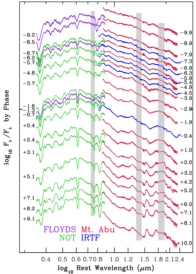
Figure 2. OIR spectra of SN 2014J from 0.32–2.4 \mu\text{m} obtained between −10d and +10d. The phases are marked at the red end for the NIR spectra and at the blue end for the optical spectra. The observatories are listed in colors that correspond to the colors of the spectra obtained at each facility. Vertical gray bars indicate regions of low atmospheric transmission.
