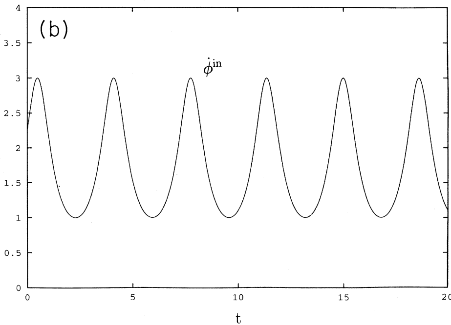
FIG. 2. In-phase state of identical-junction array. (a) shows the direction of current flow, with all horizontal junctions inactive and all vertical junctions having the same functional waveform \phi^{\text{in}}(t) ; (b) representative time series for \phi^{\text{in}}(t) .
