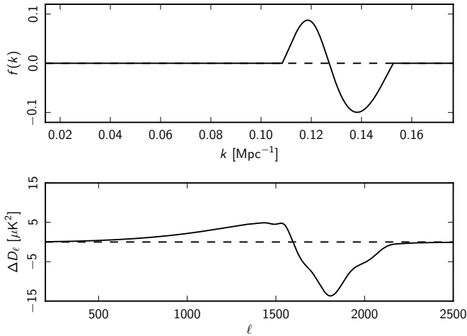
Fig. 17. CMB multipole spectrum residual for the primordial power spectrum test feature. The test feature (top) is set to the anomalously large deviation of the primordial power spectrum reconstruction for \lambda = 10^3 in the interval 0.1 \text{ Mpc}^{-1} < k < 0.15 \text{ Mpc}^{-1} , and is zero elsewhere. Bottom: the angular spectrum corresponding to this feature. We observe a large dip at \ell \approx 1800 .
