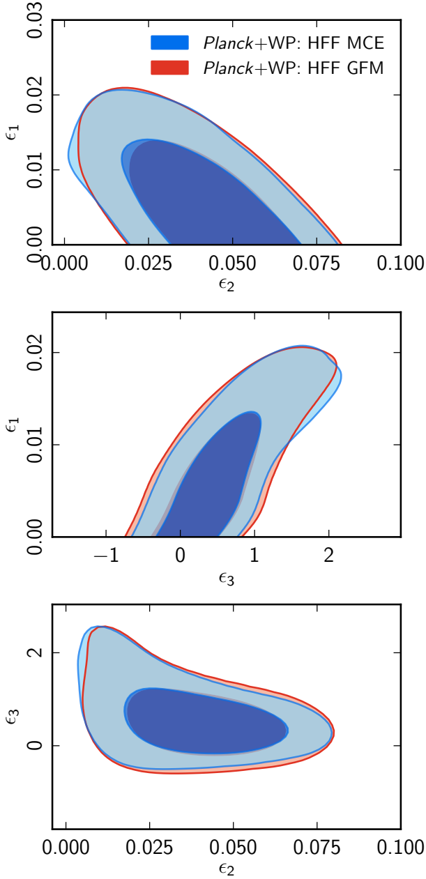
Fig. A.2. Comparison of the Planck constraints on the HFFs ( \epsilon_1, \epsilon_2, \epsilon_3 ) using the GFM and the MCE.
