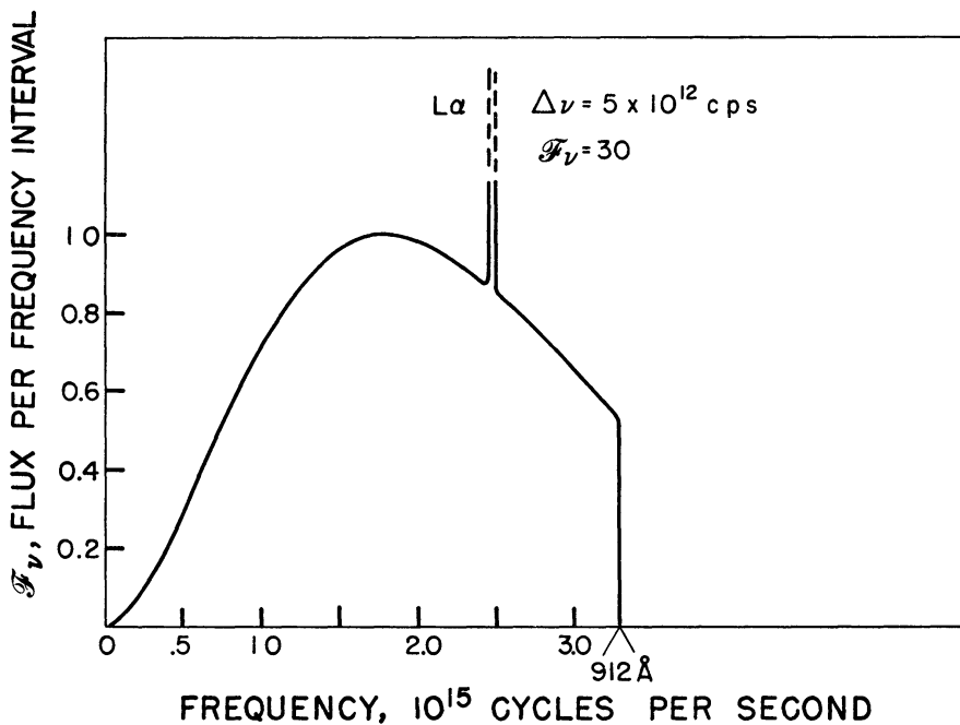
FIG. 3.—This curve represents semi-quantitatively the expected spectra of young galaxies in the extreme case that all photons of ionizing radiation have been converted to Lyman photons (§ IIIe). The expected Lyman- \alpha flux is calculated with \Delta\nu = 0.002 \nu for the line.
