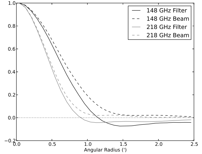
Figure 2. Matched filters (solid lines) are band pass filters that smooth the map on the scale of the beam (dashed lines) and remove large scale structure associated with the CMB, other astrophysical signals (e.g., the Sunyaev-Zel’dovich effect) and residual contamination from atmospheric brightness fluctuations. The beam and filter functions are plotted with unit normalization at their peak ( \theta = 0 ). The matched filters were binned in radius to better show the relevant angular scales. In the analysis, we use two dimensional filters to capture the anisotropic character of the noise.
