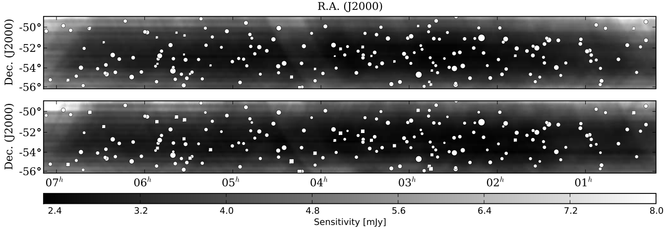
Figure 1. Sensitivity maps with source detections at 148 GHz (top) and 218 GHz (bottom), showing the most uniform 455 \text{ deg}^2 patch of the Southern strip with the greatest depth of coverage. It lies between right ascension 00^{\text{h}}12^{\text{m}} and 07^{\text{h}}07^{\text{m}} , and declination -56^{\circ}11' and -49^{\circ}00' . The deepest data correspond to an exposure time of 23.5 minutes per square arcminute and a 1\sigma sensitivity of 2.34 mJy at 148 GHz and 3.66 mJy at 218 GHz. White circles or squares mark the locations of ACT sources with a size proportional to the log of the associated source flux density. Circles denote sources designated as AGN, and squares denote sources with spectra indicative of DSFGs. Toward the edges of the map, the variation in local noise properties due to uneven coverage is more apparent.
