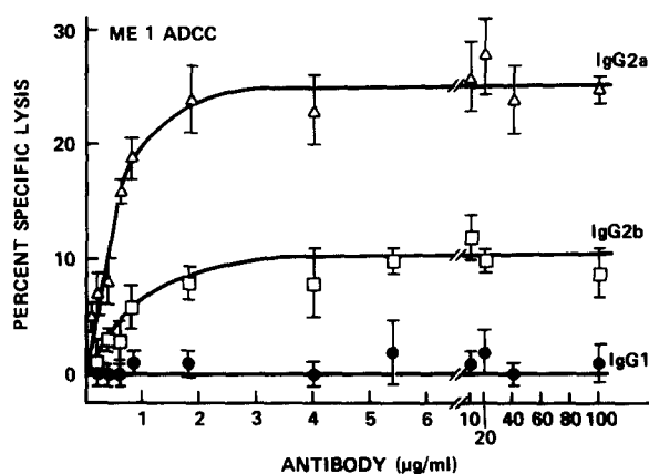
FIGURE 3. Comparison of ADCC activities of different antibody isotypes of ME1. Antibody at various concentrations was added to ^{51}\text{Cr} -labeled JY. Percent specific lysis ( \pm SD) is of JY after 4 h incubation with PBL at an E/T ratio of 50:1. IgG1 ( \bullet ), IgG2a ( \Delta ), IgG2b ( \square ).
