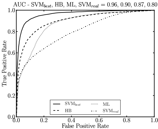
Figure 9. Receiver Operating Characteristic (ROC) curve for four photometric classification approaches: SVM_{best} , SVM_{real} , ML, and HB. The ROC curve shows the true-positive rate vs. the false-positive rate, as \ln(\Omega) varies. An ideal classifier always returns a true-positive rate of one, so the Area Under the Curve (AUC) provides a general assessment of the performance.
