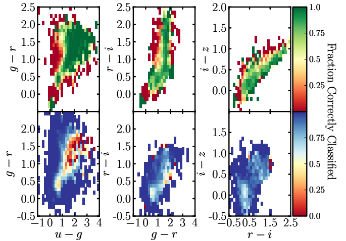
Figure 5. Fraction of objects correctly classified at \ln(\Omega) = 0 using our HB template fitting, distributed in ugriz color-color space. The top panel shows the performance on stars, and the bottom panel shows the performance on galaxies. Comparing with Figure 2, it is clear that classification is most successful for regions in which stars and galaxies do not overlap in color-color space.
