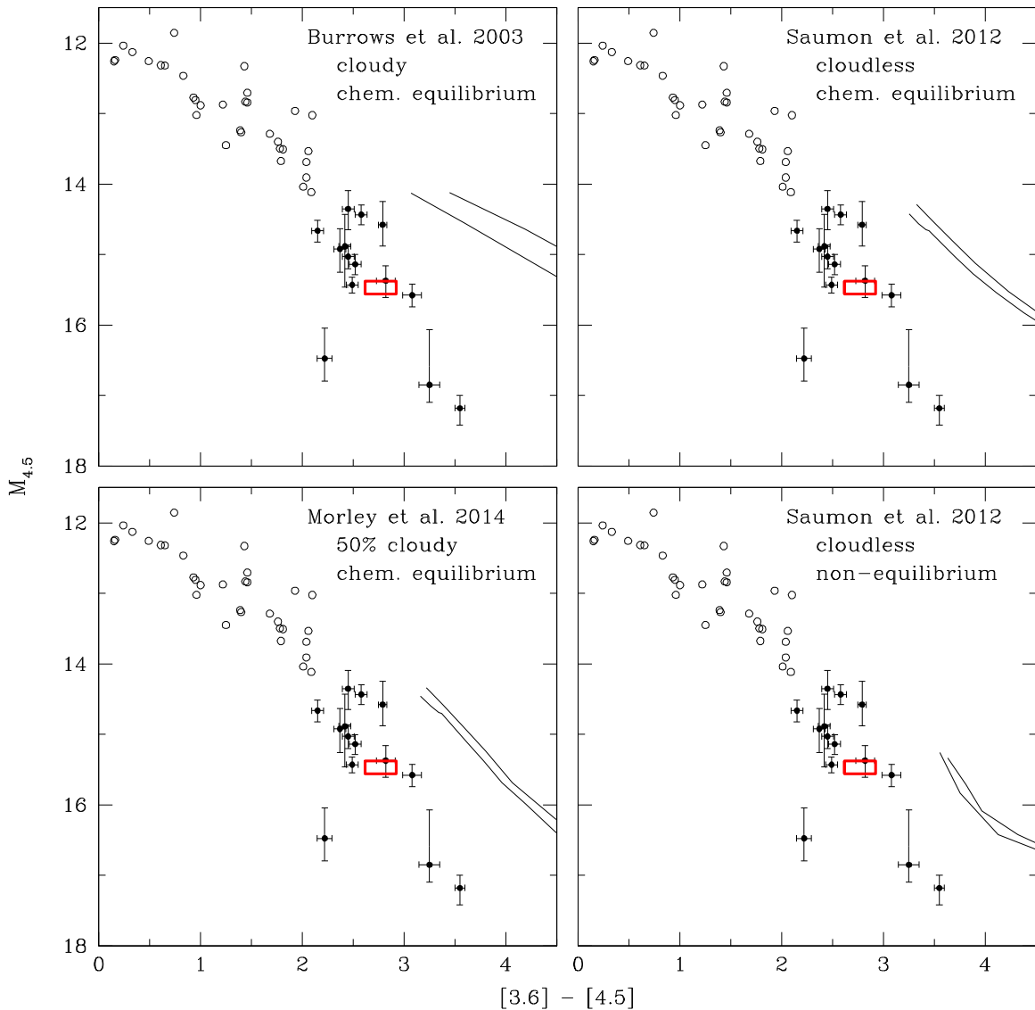
Figure 4. Same as Figure 3, except that the color is [3.6]-[4.5] . (A color version of this figure is available in the online journal.)
