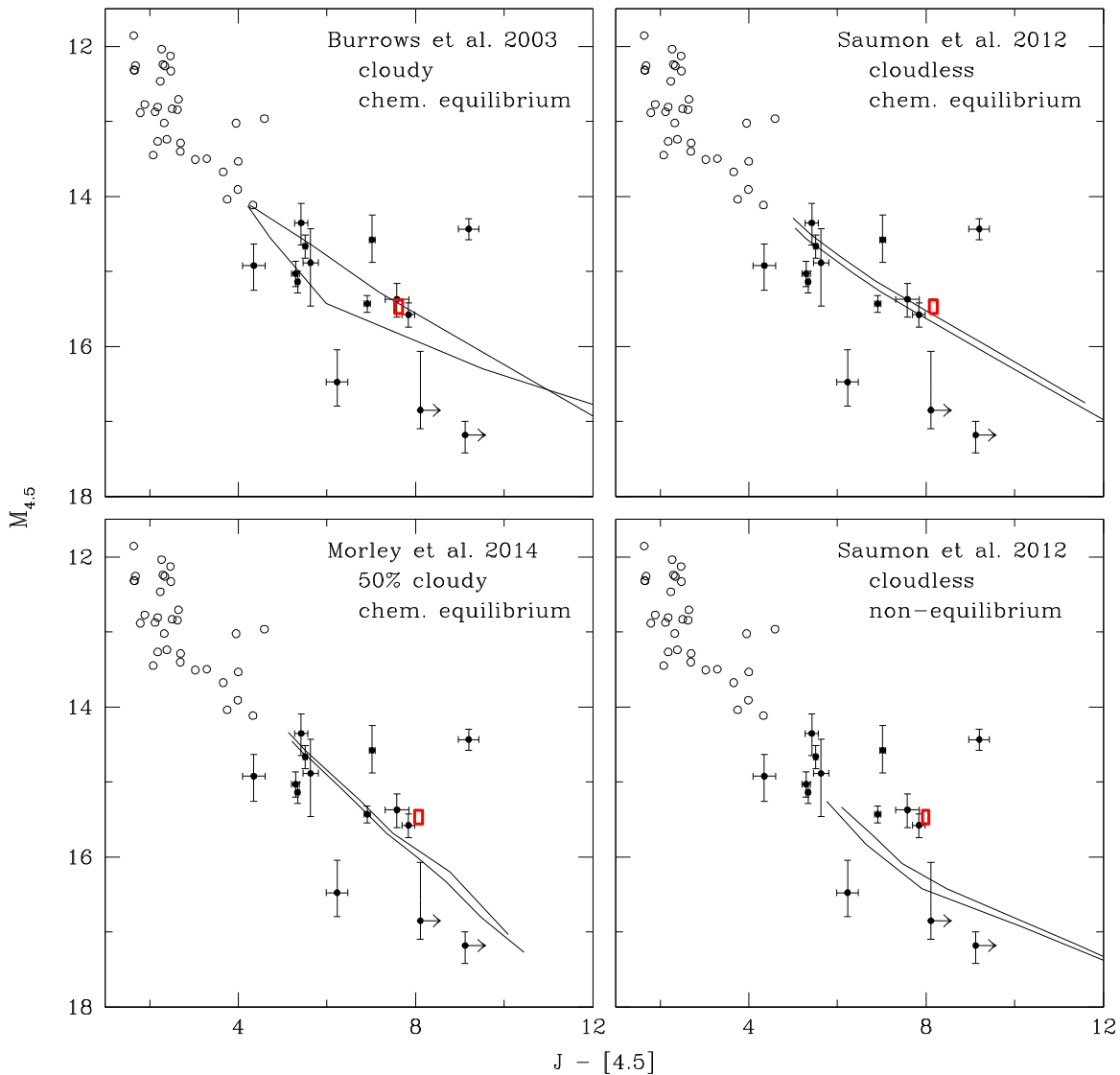
Figure 3. Color–magnitude diagrams for WD 0806-661 B (open rectangle) and samples of T dwarfs (open circles; Dupuy & Liu 2012, and references therein) and Y dwarfs (filled circles with error bars; Cushing et al. 2011, 2014; Tinney et al. 2012; Beichman et al. 2013, 2014; Leggett et al. 2013; Marsh et al. 2013; Kirkpatrick et al. 2013; Dupuy & Kraus 2013; Luhman 2014). These data are compared to the magnitudes and colors predicted by four sets of models for ages of 1 and 3 Gyr (solid lines), which encompass the age of WD 0806-661 B ( 2 \pm 0.5 Gyr; Luhman et al. 2012).
