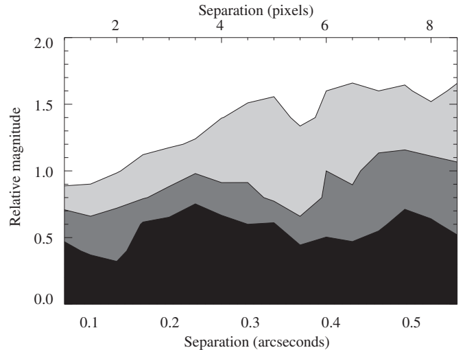
Figure 2. Relative magnitude limits at which 20%, 50%, and 80% (top to bottom) of simulated companions to WD 0806-661 B are recovered by our PSF analysis of the WFC3 F110W image.
