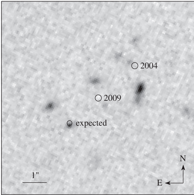
Figure 1. WFC3 F110W image of a 8'' \times 8'' field encompassing WD 0806-661 B. We have marked the positions of this object measured with Spitzer in 2004 and 2009 (Luhman et al. 2011) and the position expected in this image based on those earlier detections and the proper motion and parallax of the primary. A source is detected near the expected location, which we take to be WD 0806-661 B. The radius of each circle corresponds to 1\sigma .
