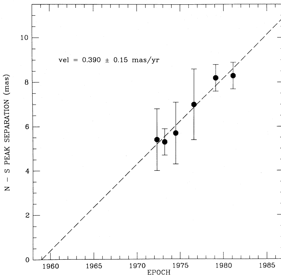
FIG. 4.—The entire size of the source, represented by the distance between the northernmost and southernmost peaks, is plotted against time. Filled circles represent the separation between the core and the southernmost peak in the 2.8 cm maps (Romney et al. 1982) where there is another peak past that extrapolated to be the knot. The error bars represent the uncertainty in identifying the correct peaks from the published 2.8 cm maps. The dashed line is a linear fit to the filled circles, v = 0.39 \pm 0.15 \text{ mas yr}^{-1} = 0.33 \pm 0.13h^{-1}c .
